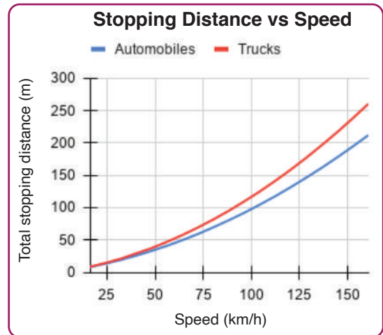
Fig. 3.8 , The plot of total stopping distance vs speed of automobiles and trucks. Data sourced from Code of Virginia, The State of Virginia.
