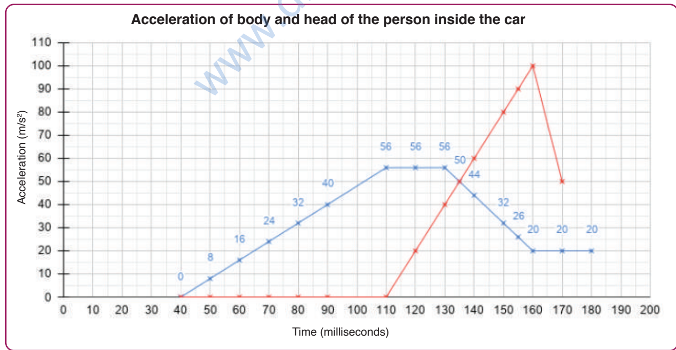
Fig. 3.9, The acceleration v/s time curve of head and torso of a person inside a car in a simulation of a rear-end collision
