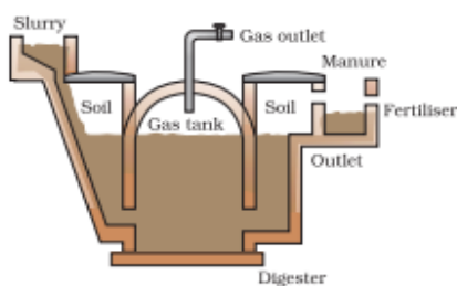
Figure 14.4 Schematic diagram of a bio-gas plant
