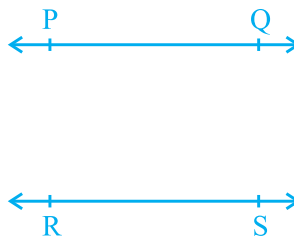
(ii) Non-intersecting (parallel) lines
