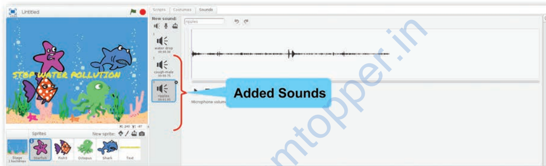
Fig. 8.12: Adding sound
