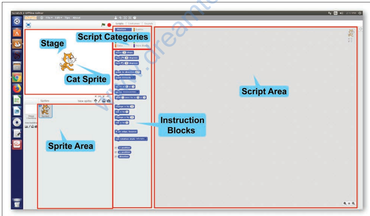
Fig. 8.3: Scratch Interface
