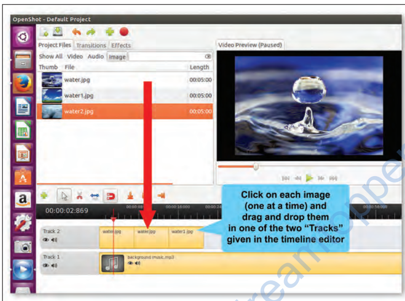
Fig. 4.10: Adding images on the timeline (Method 1)
