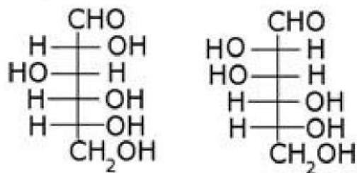
D - Glucose
