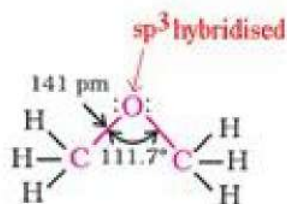
Methoxymethane (Ether)
