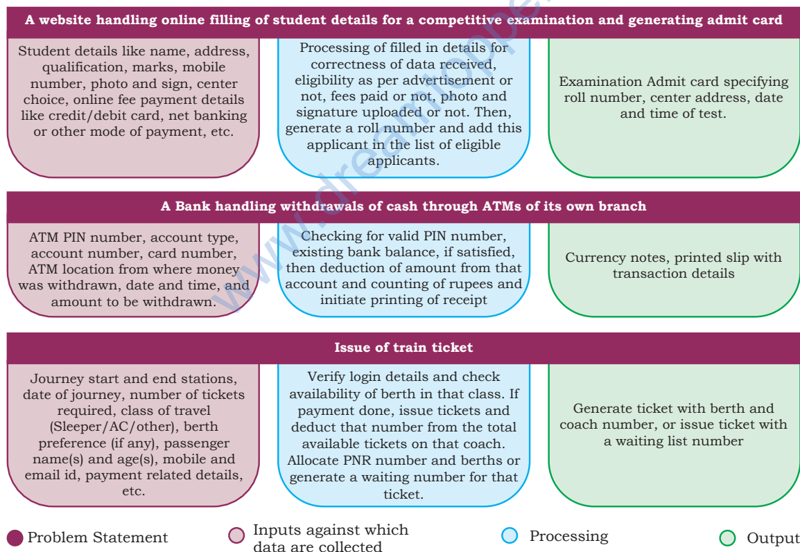
Figure 5.2: Data Based Problem Statements
