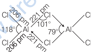
Dimer structure of AlCl_3 ( Al_2Cl_6 )
