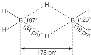
Structure of diborane
