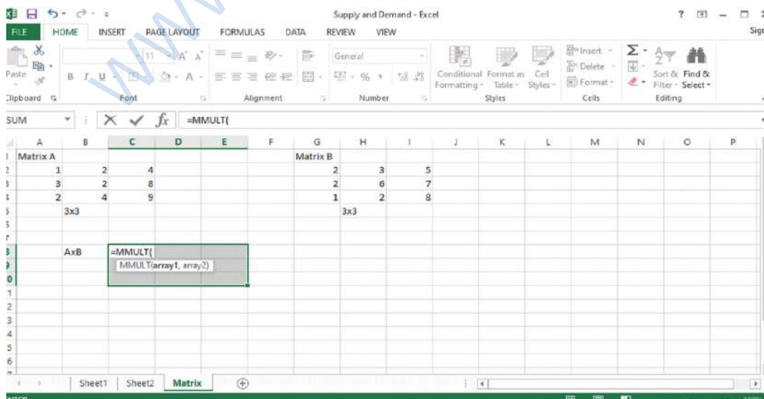
Fig 6: MMULT () function
