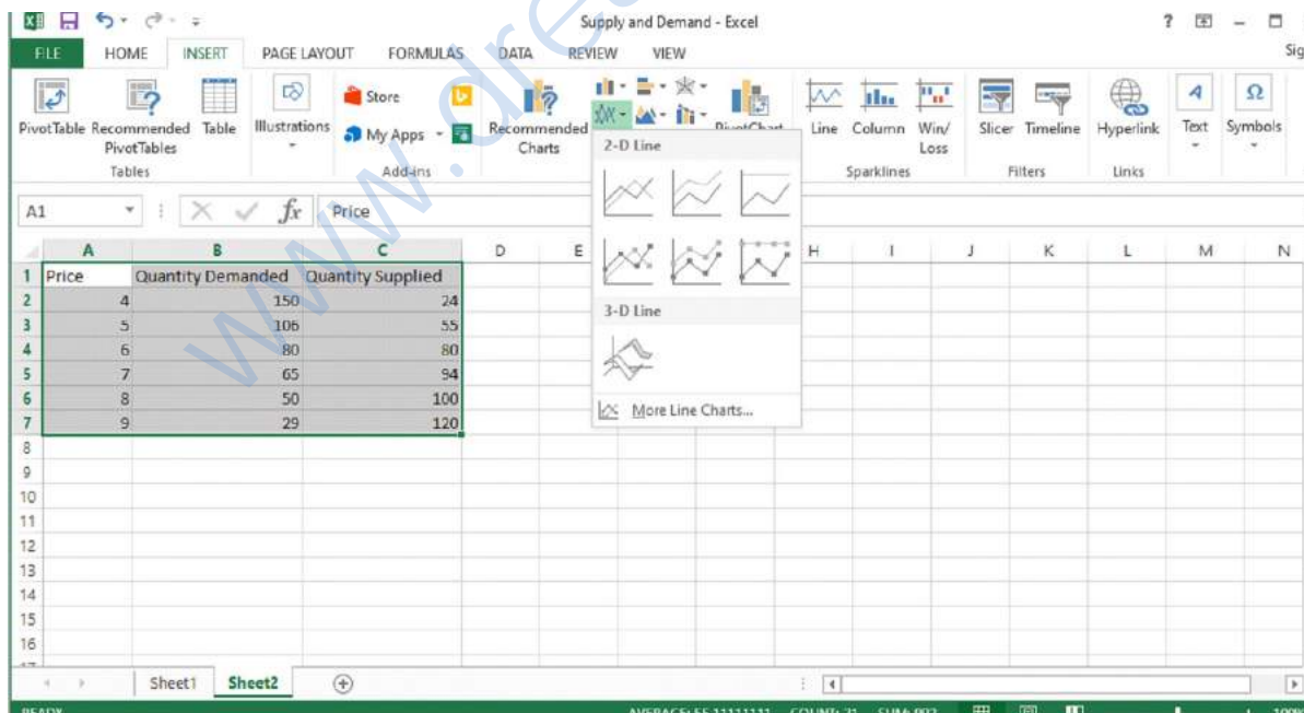
Fig 2: Line Chart
