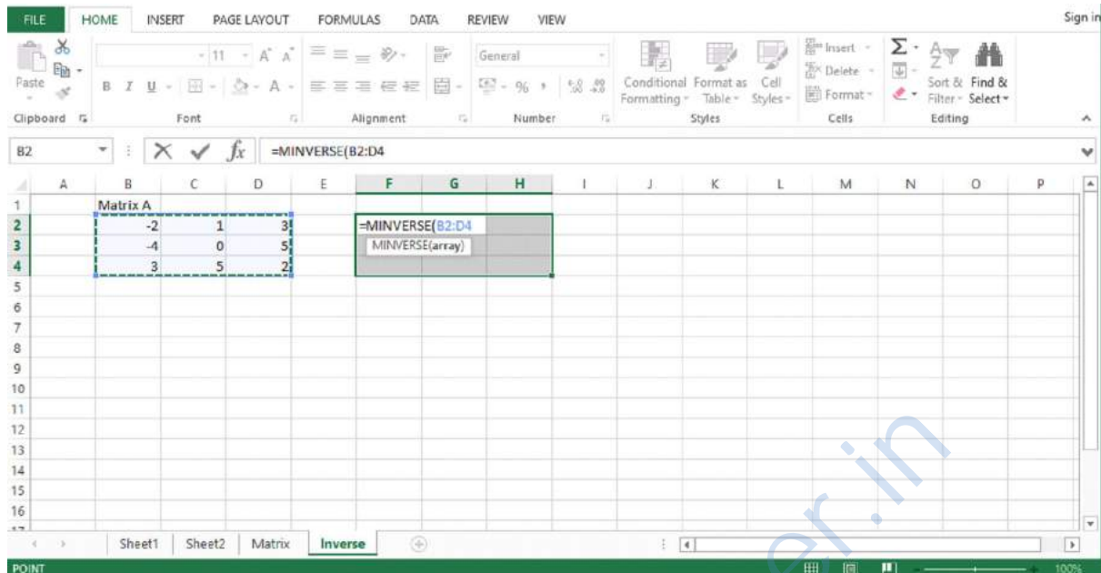
Fig 11: MINVERSE Function
