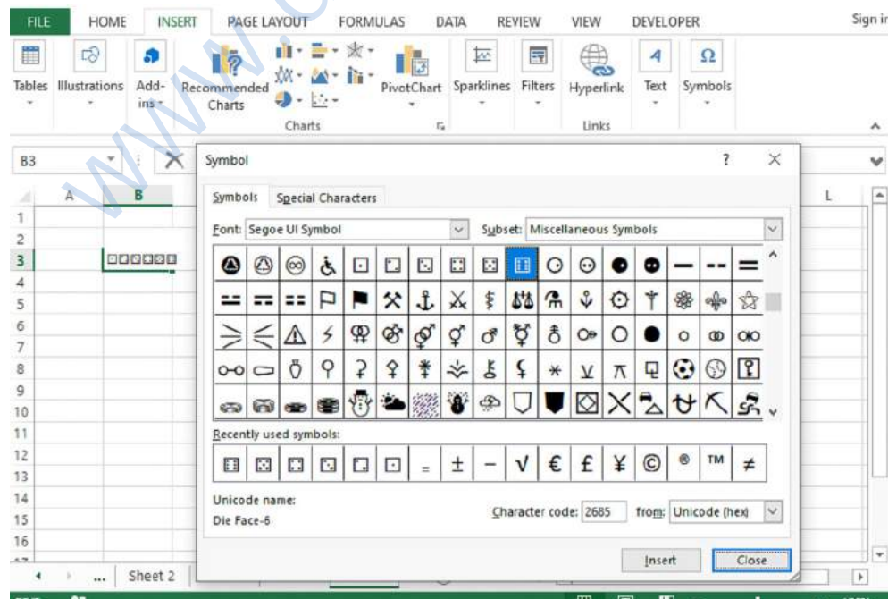
Fig 17: Dices
