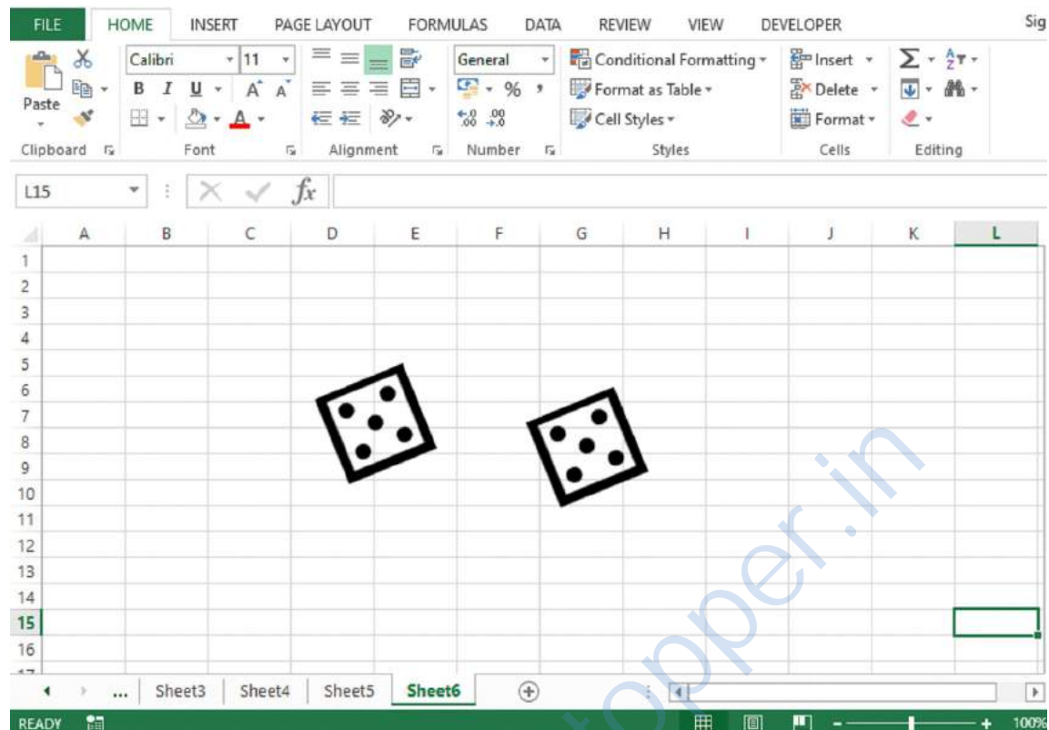
Fig 29: Two dices
