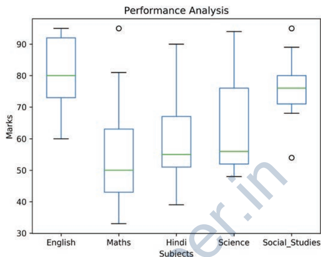
Figure 4.17: A boxplot of “Marks.csv”
