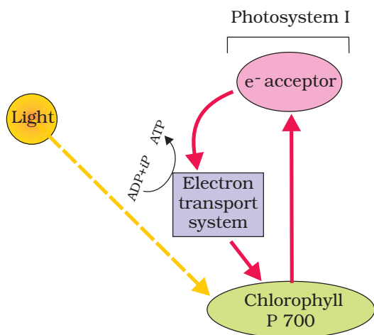
Figure 11.6 Cyclic photophosphorylation
