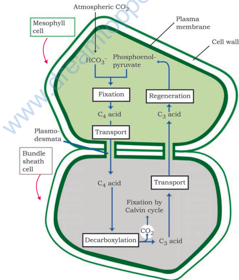
Figure 11.9 Diagrammatic representation of the Hatch and Slack Pathway
