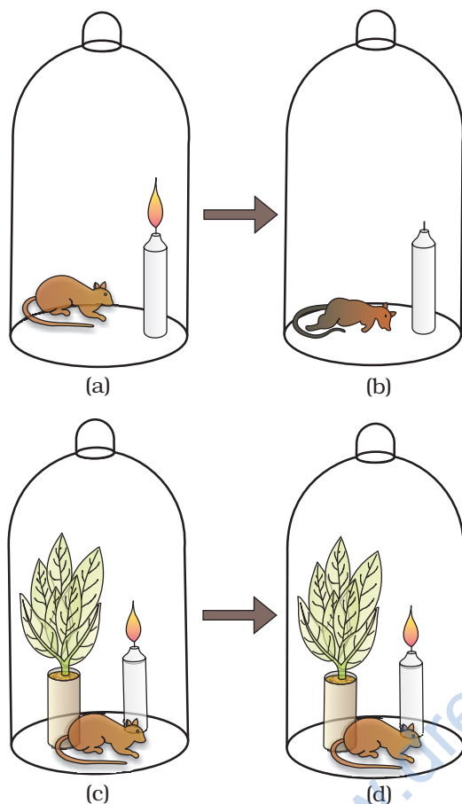
Figure 11.1 Priestley's experiment
