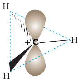
Fig. 8.3(a) Shape of methyl carbocation
