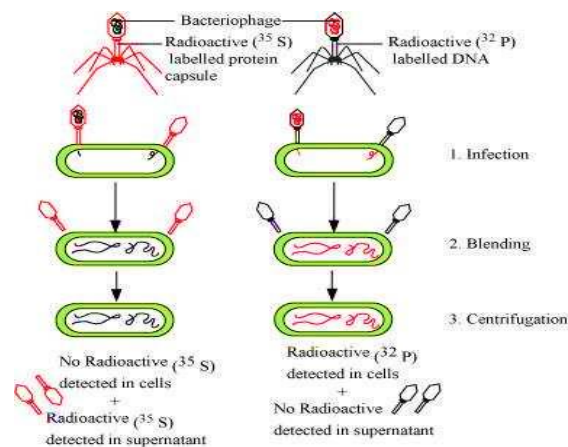
Hershey and Chase experiment
