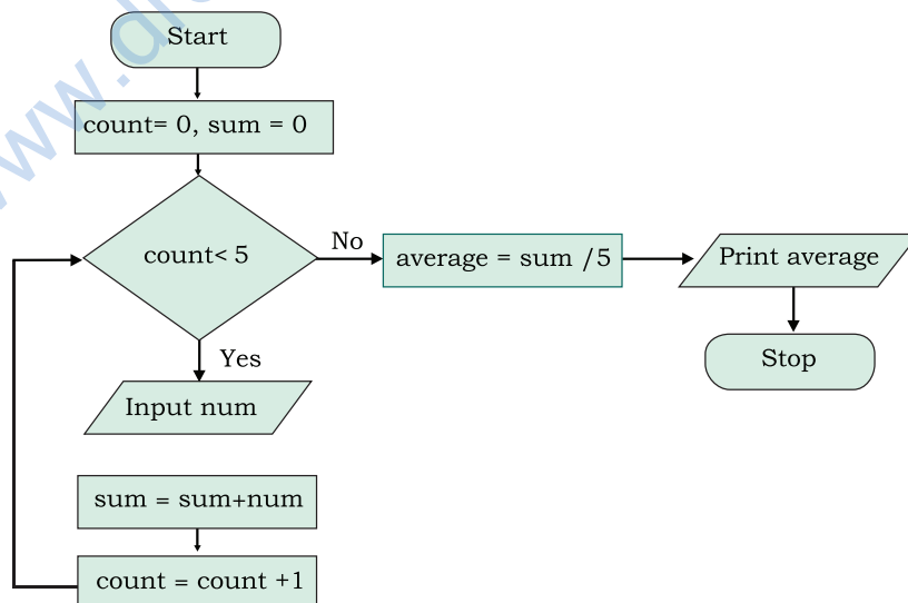
Figure 4.10: Flowchart to Calculate the Average of 5 Numbers
