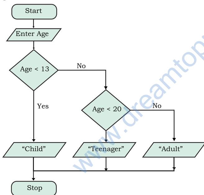
Figure 4.9: Flowchart to check multiple conditions
