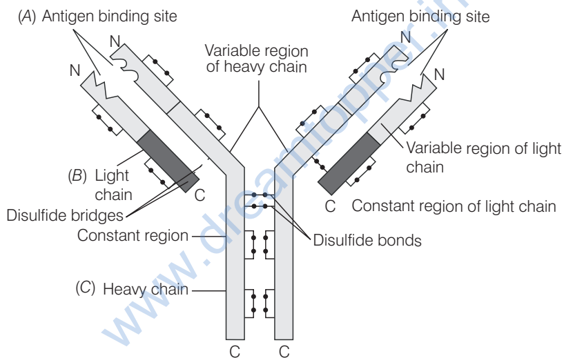
Structure of an antibody molecule
