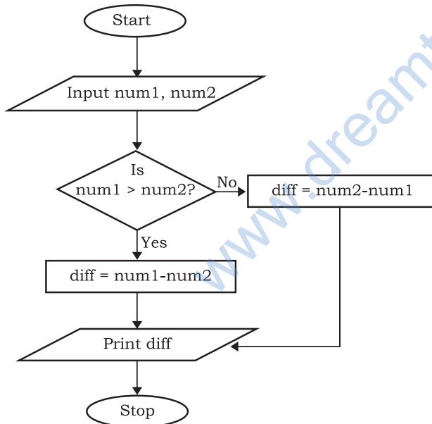
Figure 6.2: Flow chart depicting decision making
