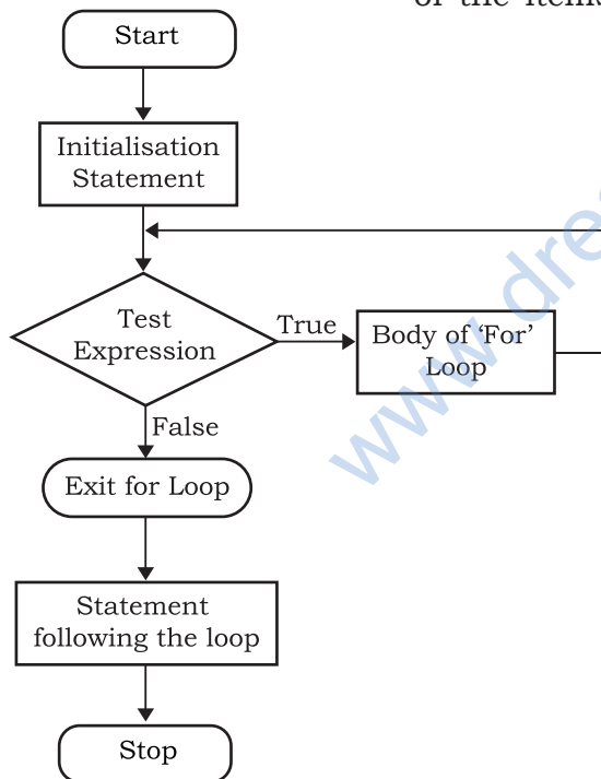
Figure 6.4: Flow chart of for loop
