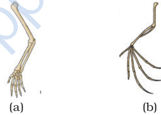
Fig. 25.8 Fore limb of (a) human (b) bat
