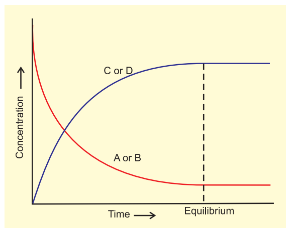
Fig. 6.2 Attainment of chemical equilibrium.
