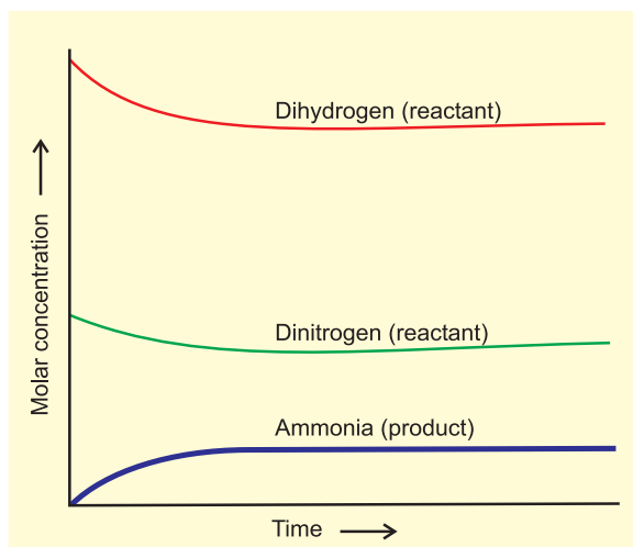
Fig. 6.4 Depiction of equilibrium for the reaction
