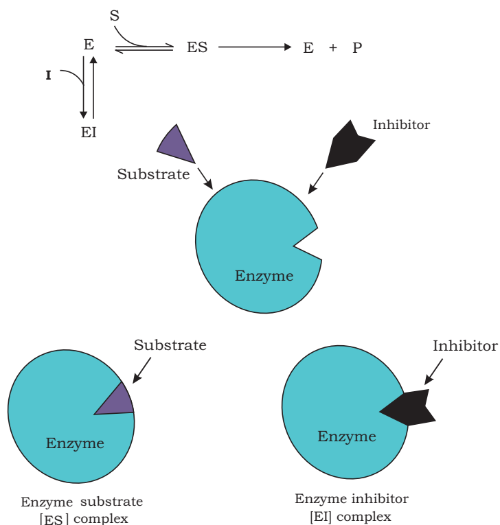
Fig. 4.7: Competitive inhibition
