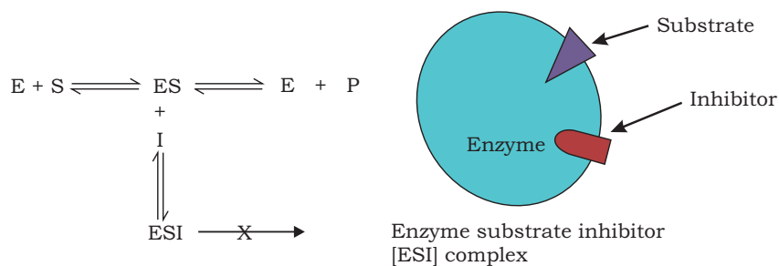
Fig. 4.11: Uncompetitive inhibition
