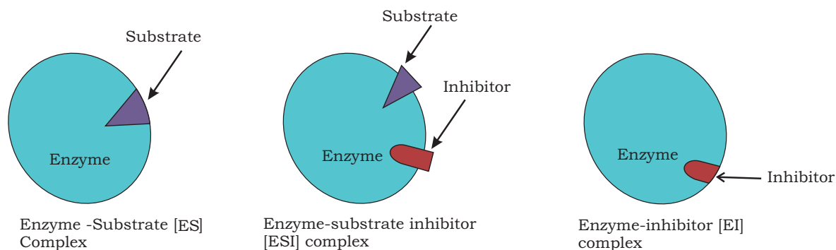
Fig. 4.9: Non-competitive inhibition
