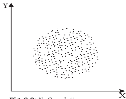
Fig. 6.3: No Correlation
