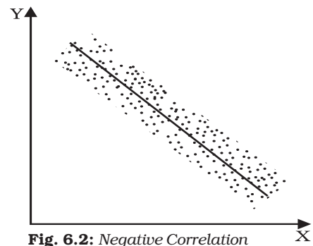
Fig. 6.2: Negative Correlation
