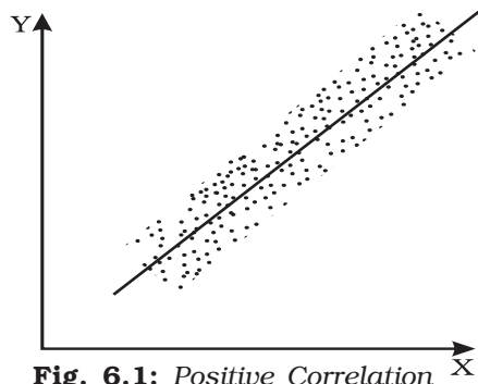
Fig. 6.1: Positive Correlation
