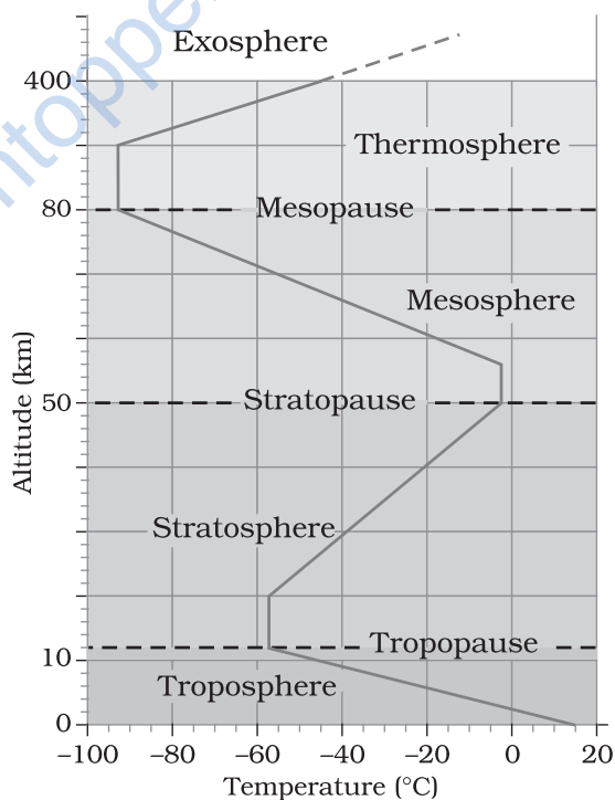
Figure 7.1 : Structure of atmosphere
