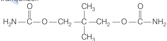
Structure of equanil
