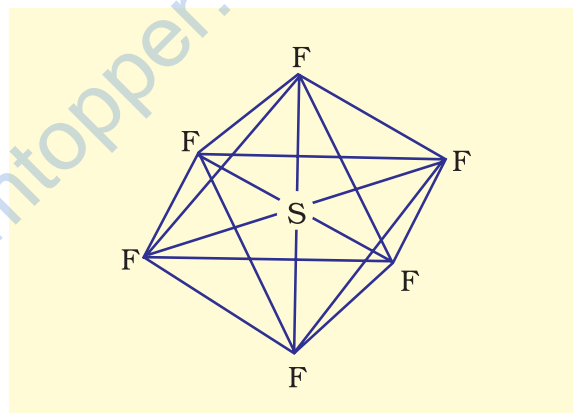
Fig. 4.18 Octahedral geometry of SF_6 molecule
