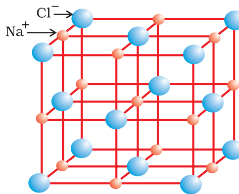
Rock salt structure
