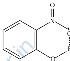
Fig. 4.22 Intramolecular hydrogen bonding in o -nitrophenol molecule
