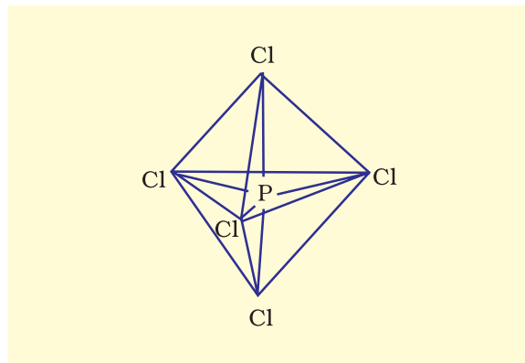
Fig. 4.17 Trigonal bipyramidal geometry of PCl_5 molecule
