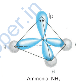
Fig.4.13 Formation of \text{NH}_3 molecule
