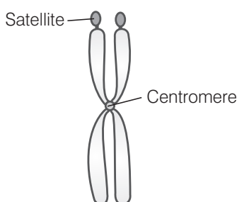
Diagram representing satellite chromosomes
