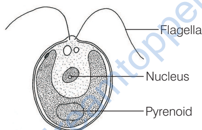
Zoospore of Chlamydomonas
