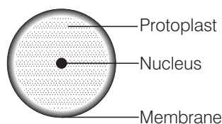
Aplanospore of Spirogyra
