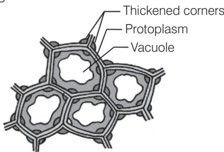
Collenchyma cells
