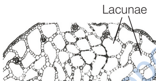
Aerenchyma cells
