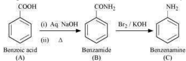
Benzoic acid
